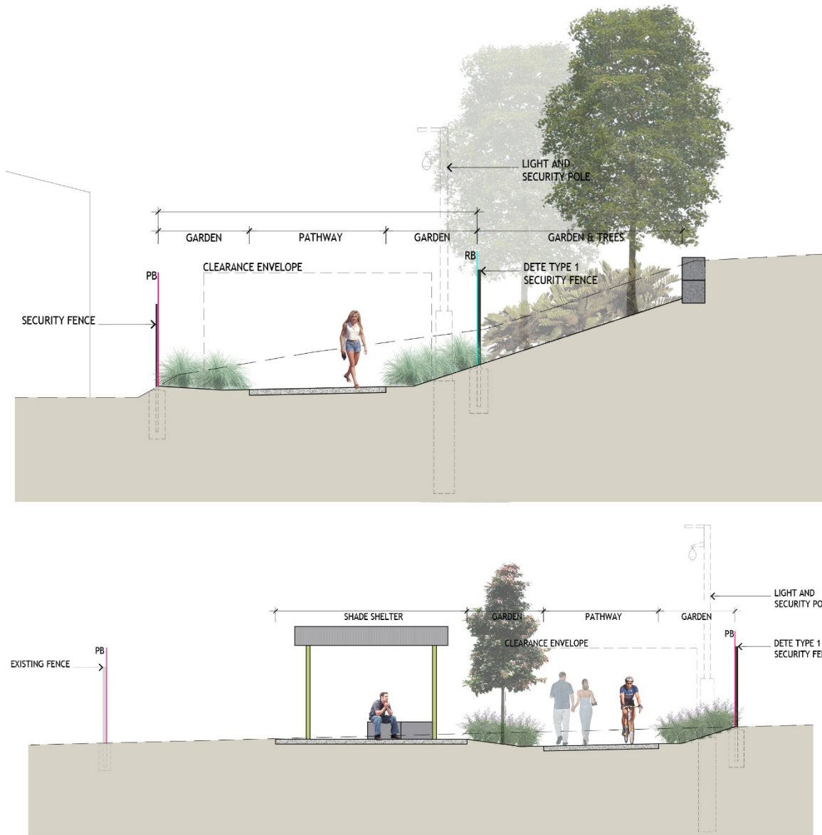
Figure 1 - Murrajong Road to Dennis Road Shared Pathway Concept design (sections)
